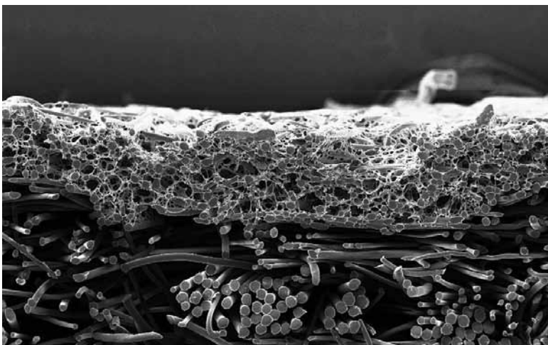
Novates felt-detail
