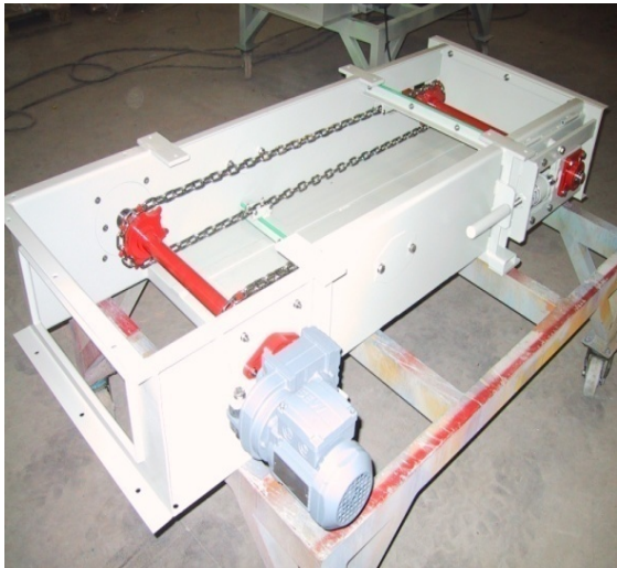
REDLER TYPE SPILLAGE CONVEYOR
